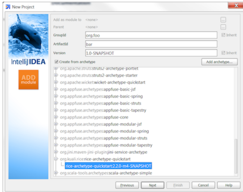
Figure 5.19. Select archetype
