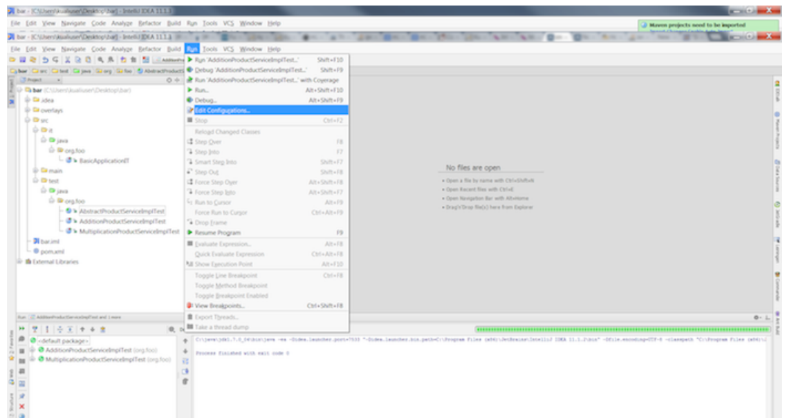
Figure 5.26. Edit configurations
