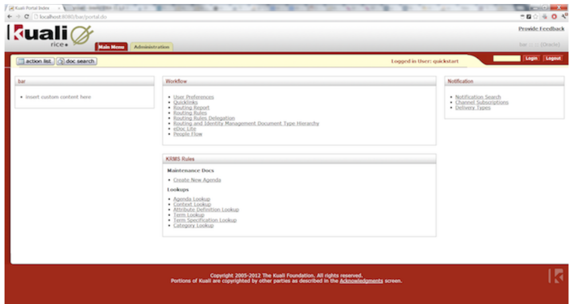
Figure 5.15. Initial screen
