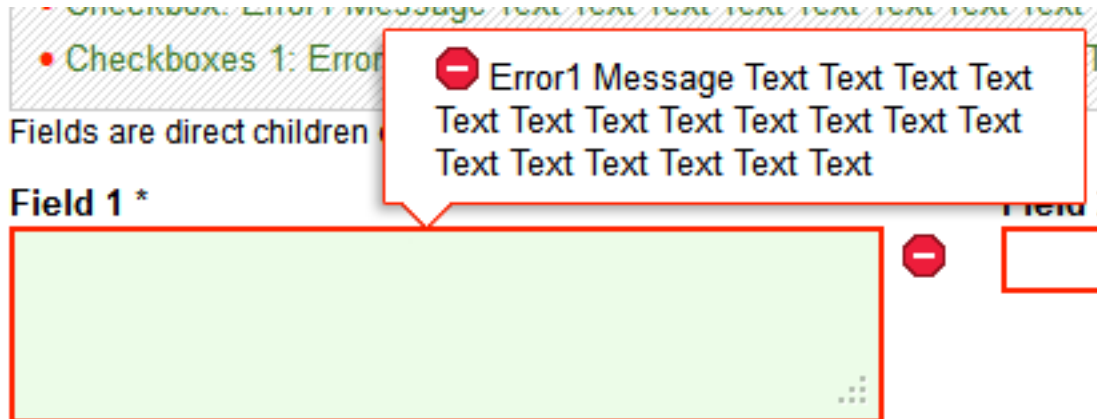
Figure 7.30. ValidationMessages for an InputField
