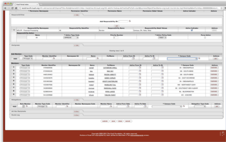
Figure 14.6. Role Screen, Qualifiers
