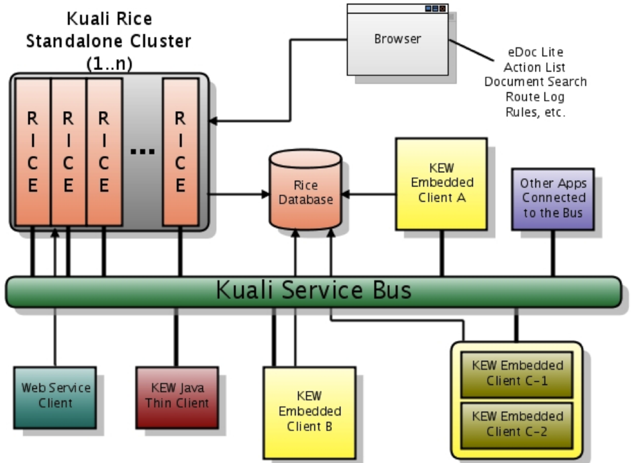
Figure 3.1. Kuali Rice 2.5.5 Architectural Diagram
