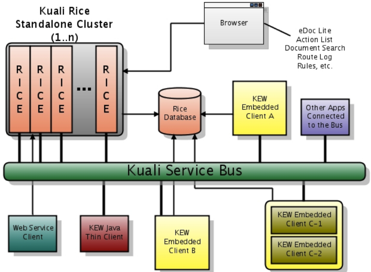
Figure 3.1. Kuali Rice 2.5.4-SNAPSHOT Architectural Diagram
