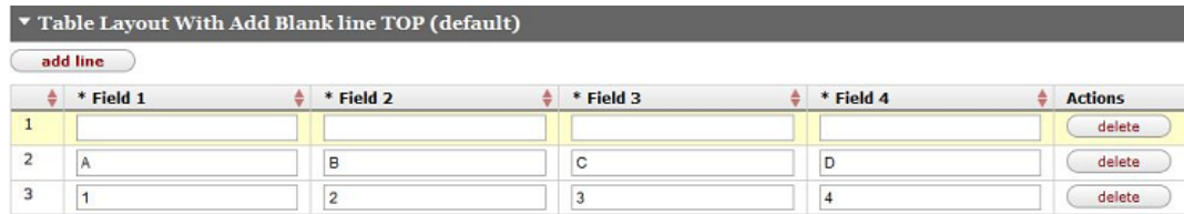
Figure 8.20. Collection Add Blank Line Example - TableLayout with TOP add line placement
