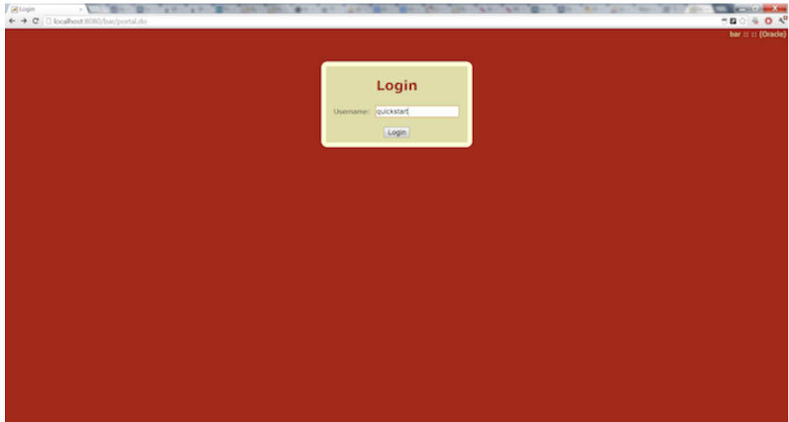
Figure 6.14. Eclipse: Login
