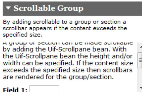
Figure 8.26. Scrollable Section
