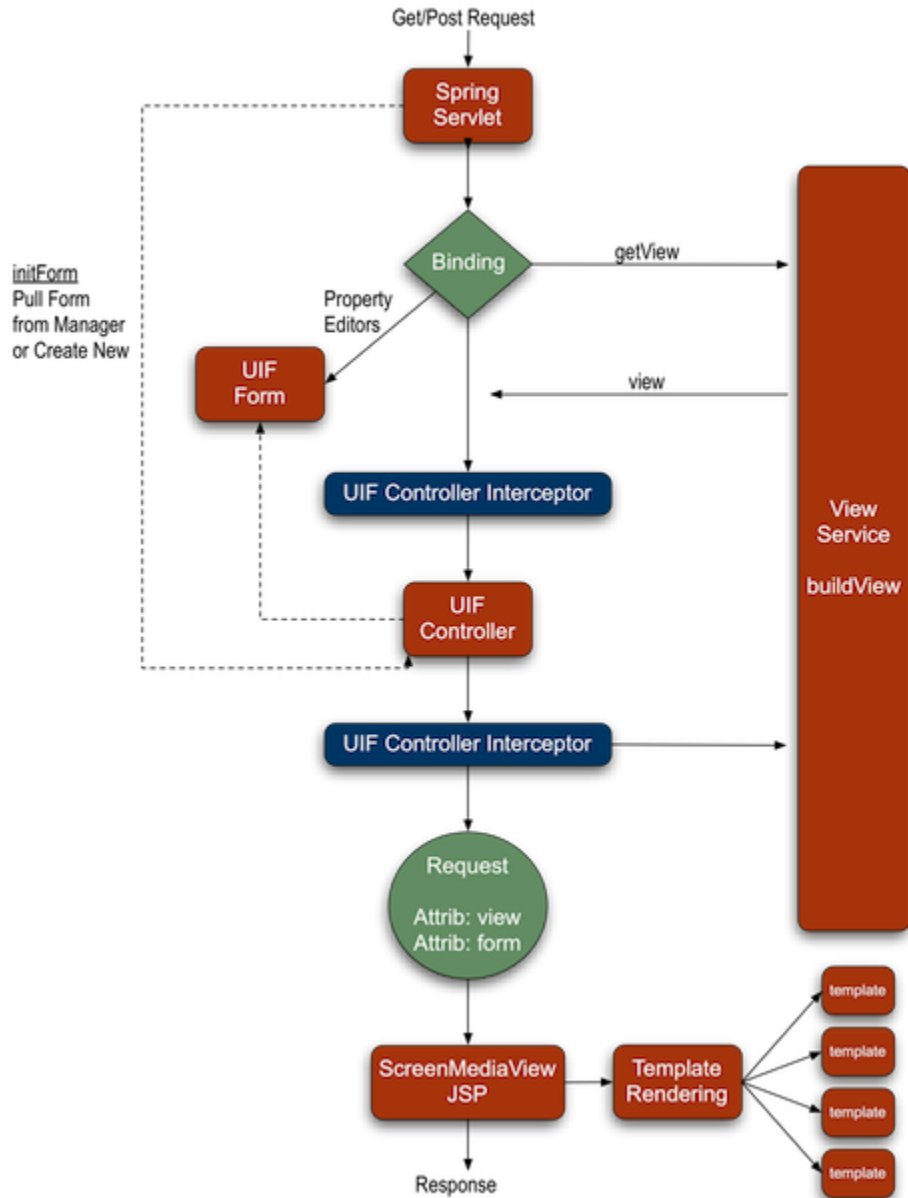
Figure 10.4. RequestResponseFlow
