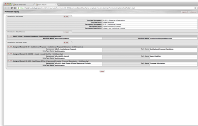
Figure 14.7. Permission Inquiry
