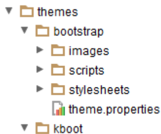
Figure 10.7. Theme Directory Structure
