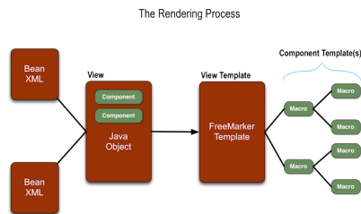
Figure 6.4. KRAD Rendering Process
