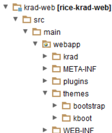
Figure 10.6. KRAD Web Structure
