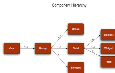
Figure 6.6. KRAD Component Hierarchy
