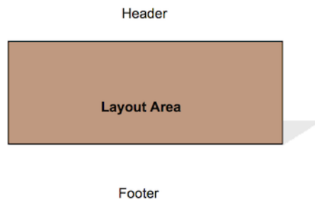
Figure 8.9. Group Layout
