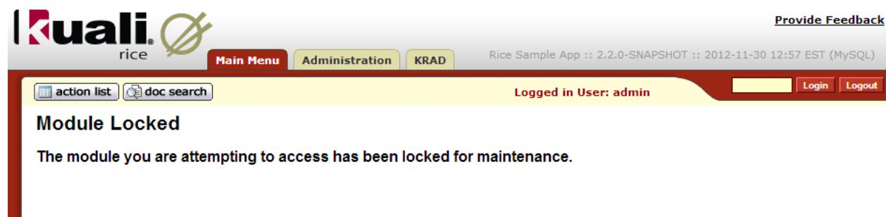
Figure 14.9. Message View
