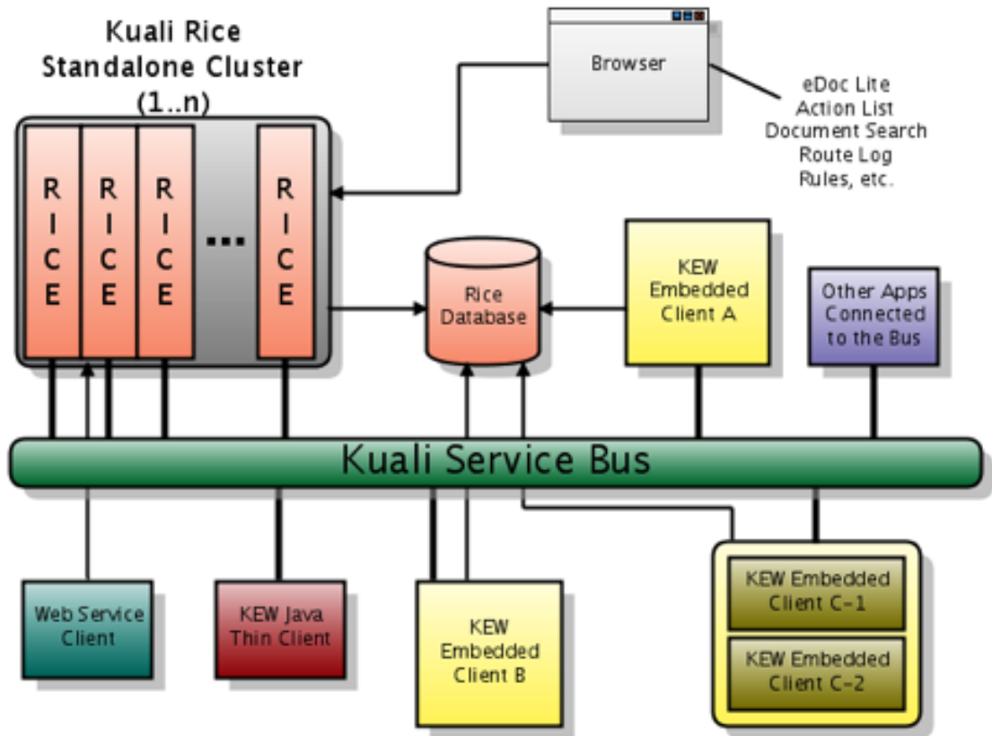
Figure 9.4. Typical enterprise deployment of Kuali Rice
