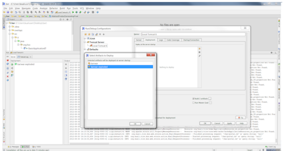
Figure 5.27. IntelliJ: Deploy
