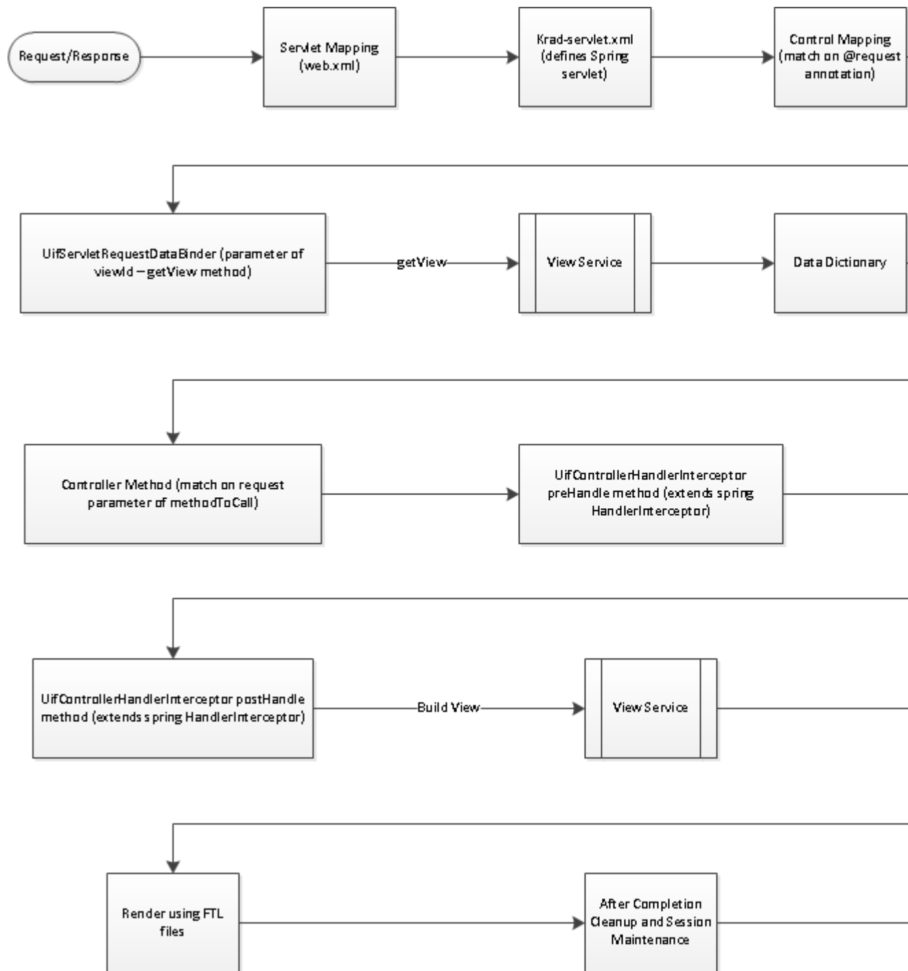
Figure 9.5. Detailed RequestResponseFlow
