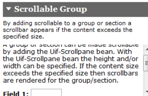
Figure 7.25. Scrollable Section
