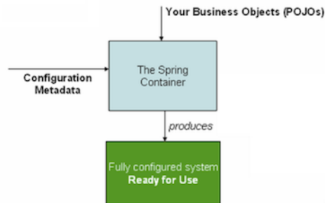
Figure 2.2. Bean Factories
