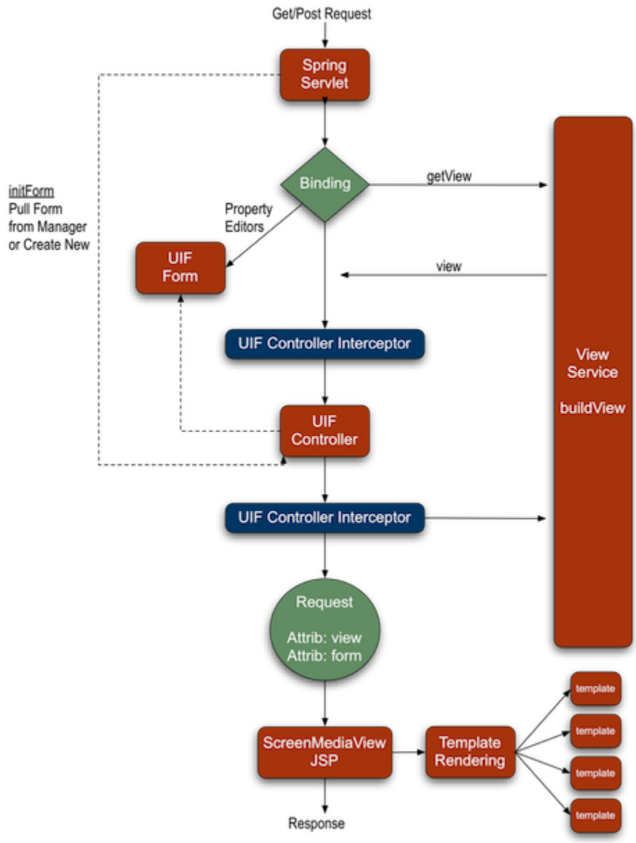
Figure 9.4. RequestResponseFlow
