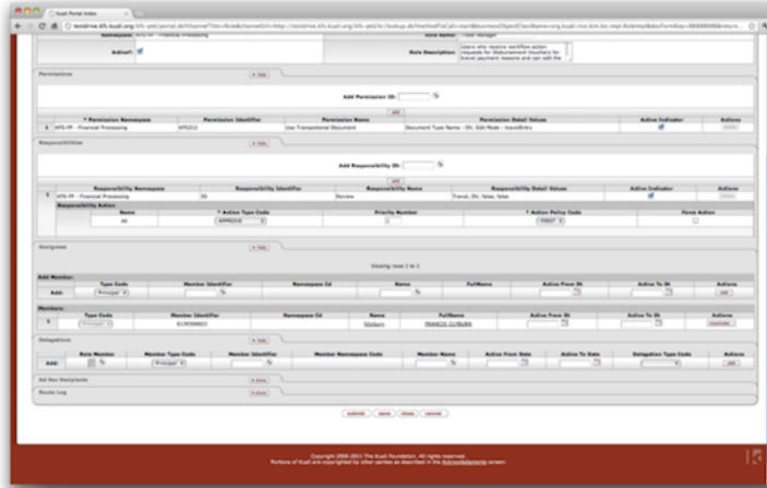
Figure 13.3. Role Screen
