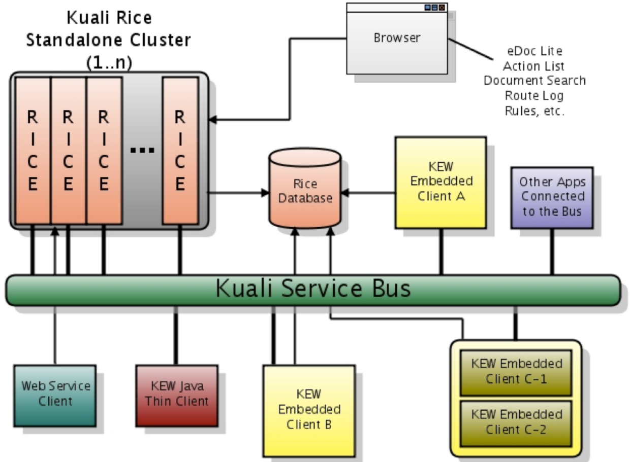
Figure 3.1. Kuali Rice 2.4.1-SNAPSHOT Architectural Diagram
