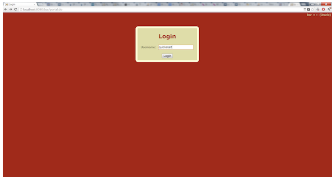
Figure 5.14. Eclipse: Login
