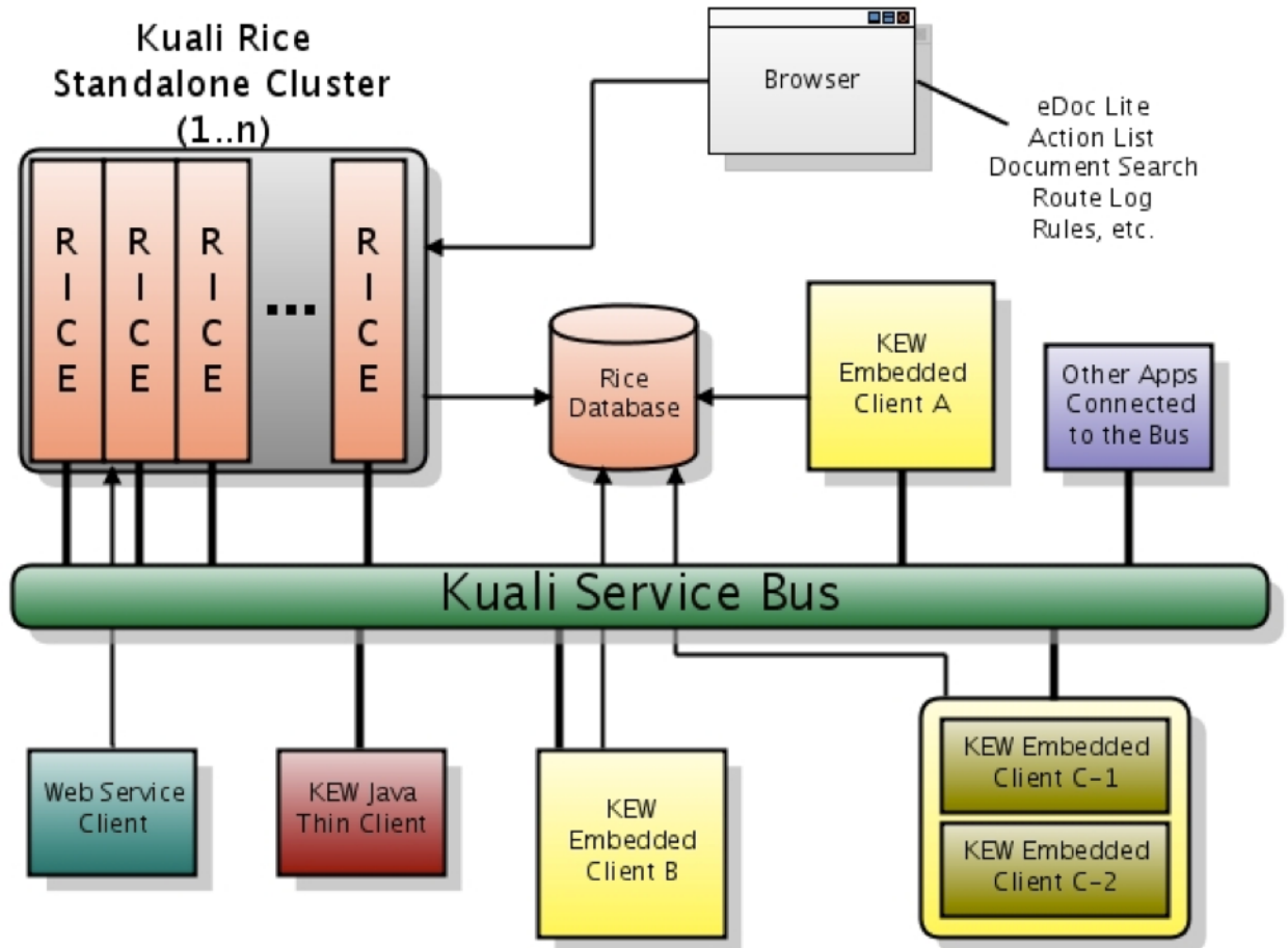
Figure 3.1. Kuali Rice 2.4.0-M2-SNAPSHOT Architectural Diagram
