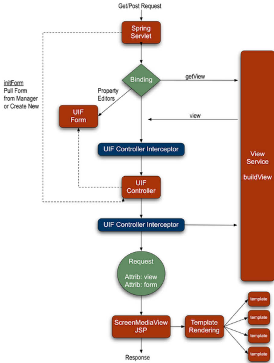
Figure 9.4. RequestResponseFlow
