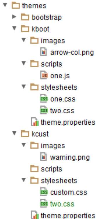
Figure 9.8. Parent/Child Theme Directories
