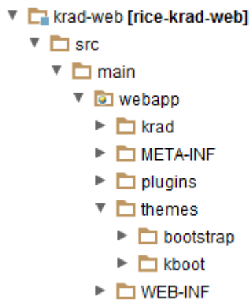
Figure 9.5. KRAD Web Structure
