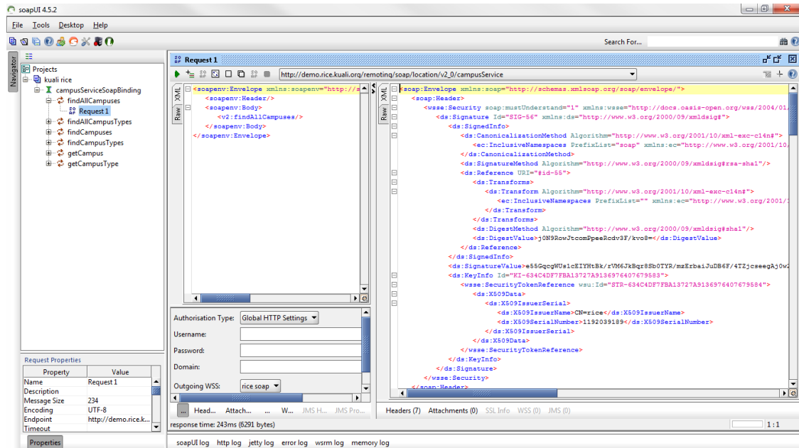
Figure 22.5. Execute request
