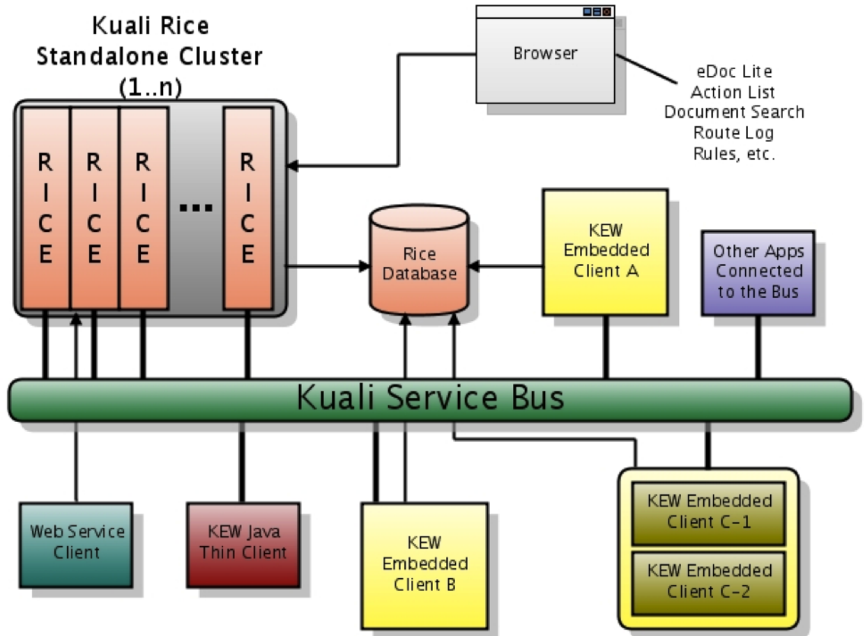
Figure 3.1. Kuali Rice 2.3.11 Architectural Diagram
