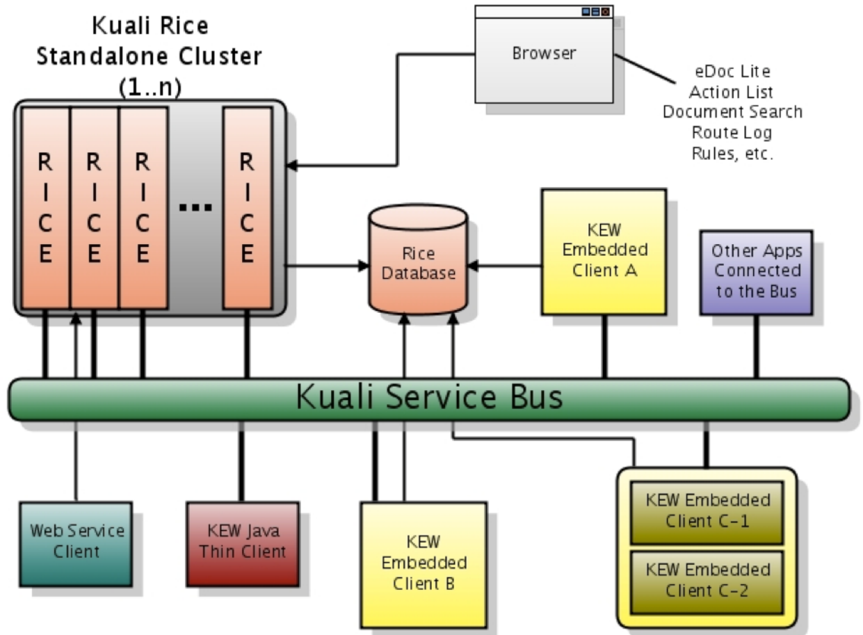
Figure 3.1. Kualu Rice 2.3.1-SNAPSHOT Architectural Diagram
