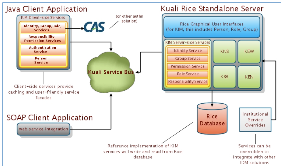
Figure 1.1. KIM Architecture
