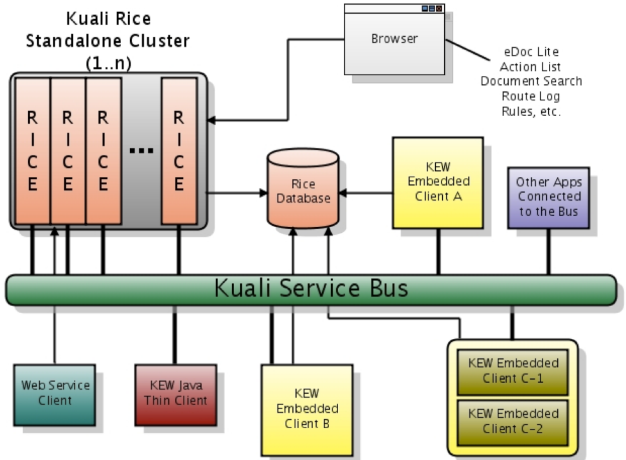
Figure 3.1. Kuali Rice 2.3.0-rc3-SNAPSHOT Architectural Diagram
