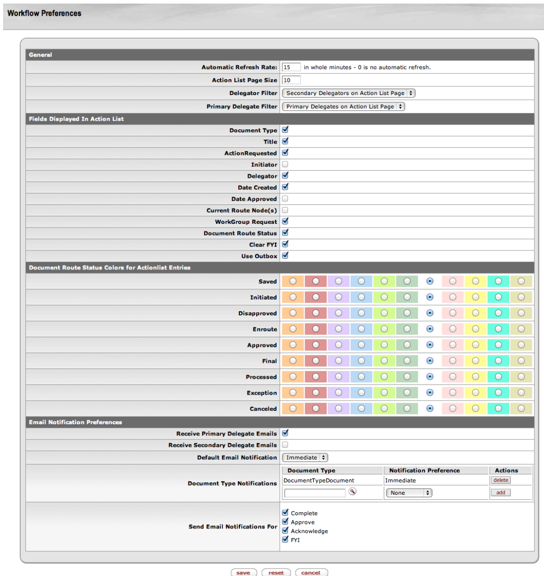
Figure 3.5. Action List Preference Page
