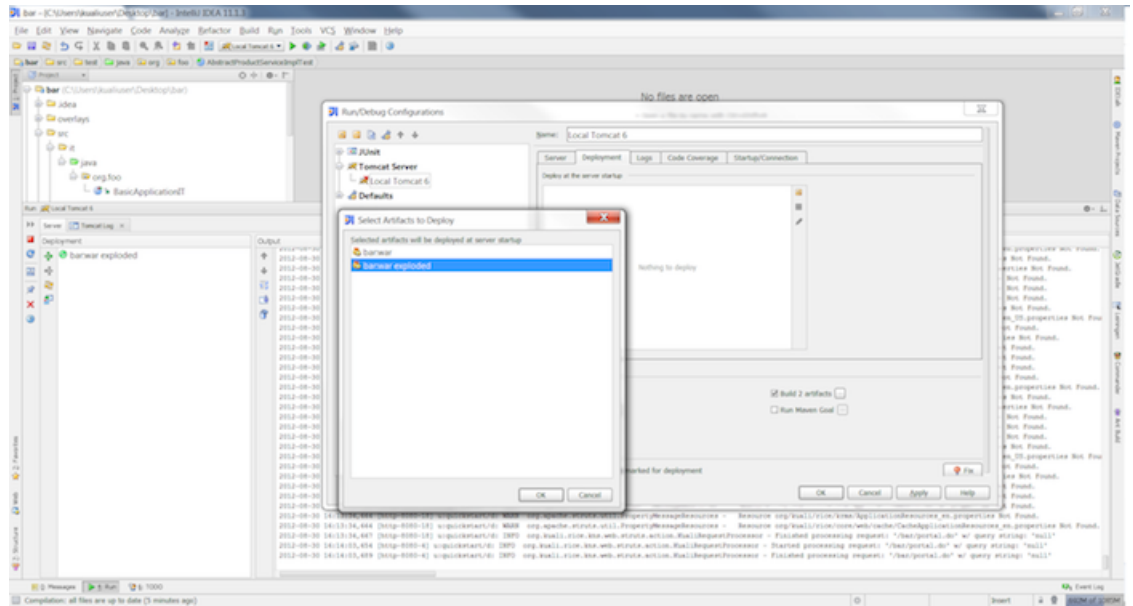
Figure 5.29. IntelliJ: Deploy
