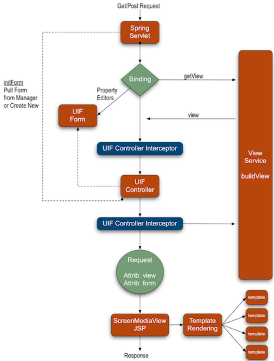
Figure 9.2. RequestResponseFlow
