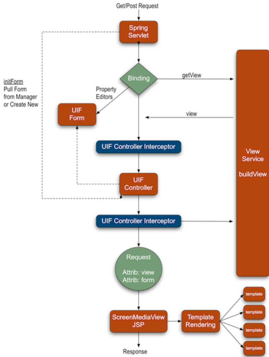
Figure 9.2. RequestResponseFlow
