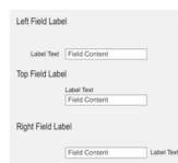
Figure 6.1. labelPlacement Options
