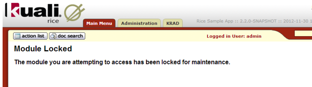
Figure 13.7. Message View
