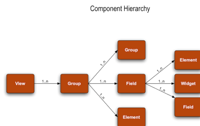
Figure 5.3. KRAD Component Hierarchy
