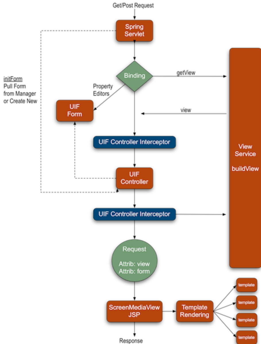
Figure 9.2. RequestResponseFlow
