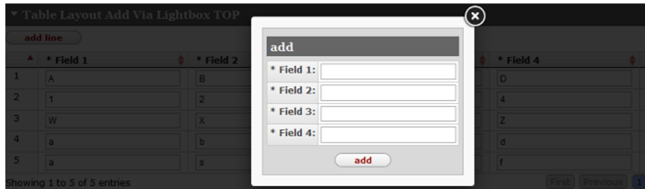
Figure 7.19. Collection Add Via Lightbox Example - TableLayout with TOP add line placement
