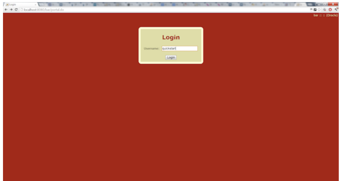
Figure 5.32. Login
