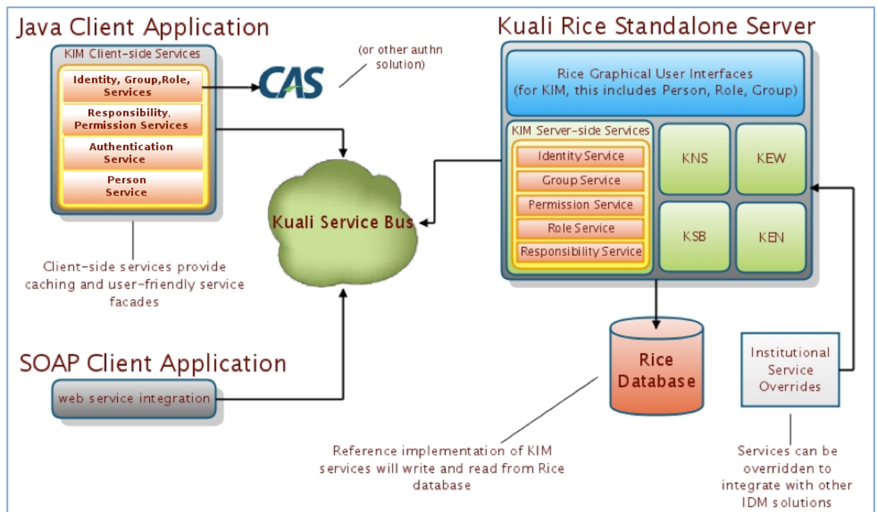
Figure 5.1. KIM Architecture
