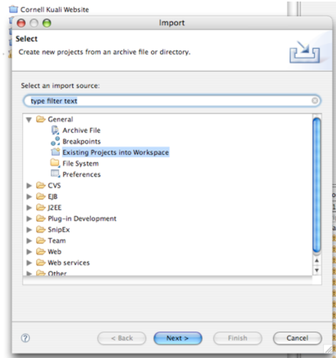
Figure 5.1. Eclipse Import
