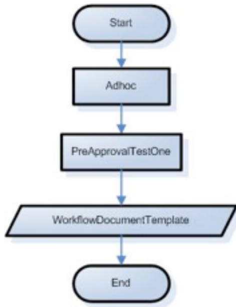
Figure 3.19. PreApproval Test
