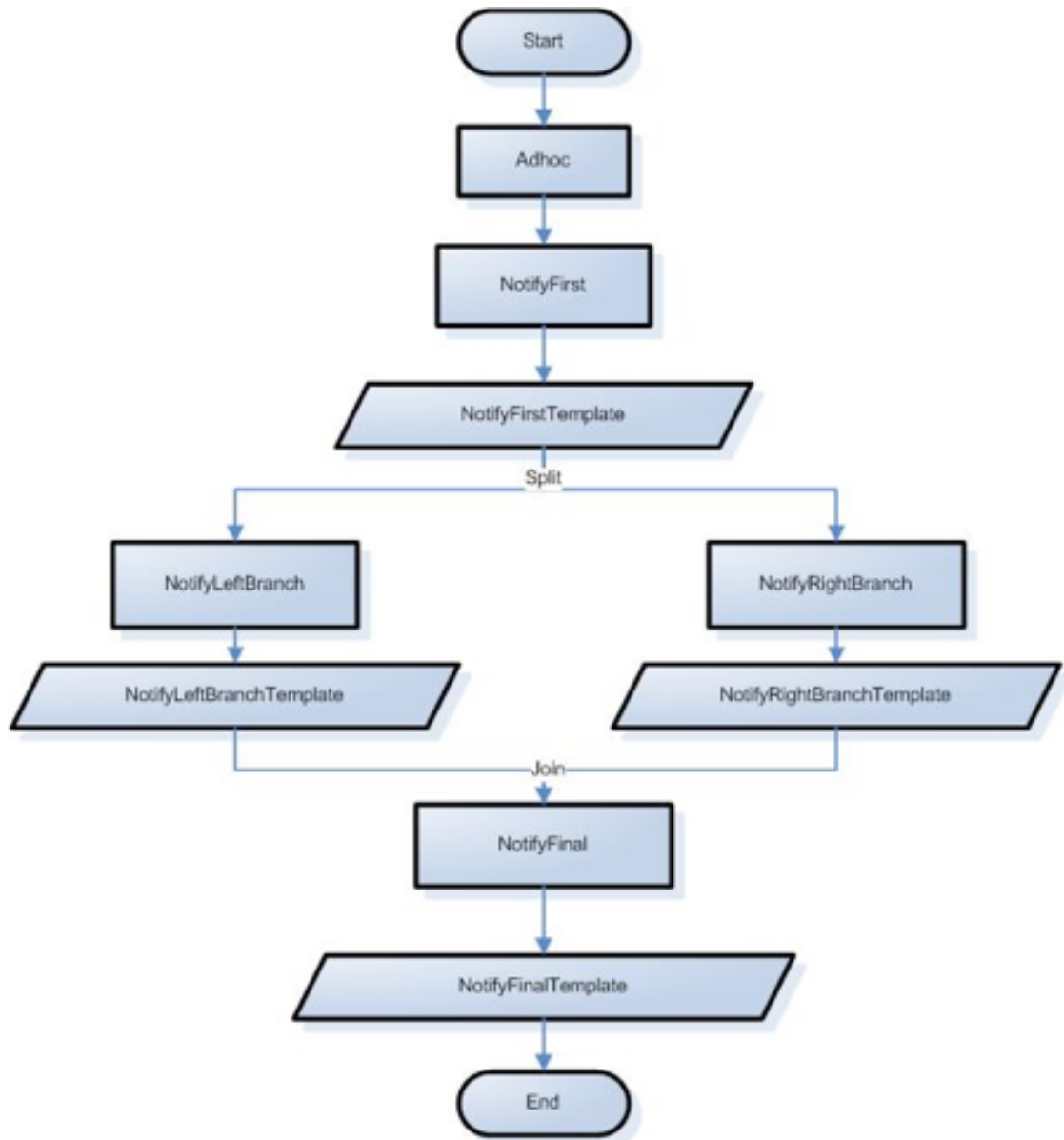
Figure 3.11. NotificationTest Workflow
