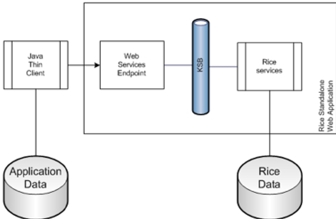
Figure 1.3. Diagram of a sample Thin Java Client implementation
