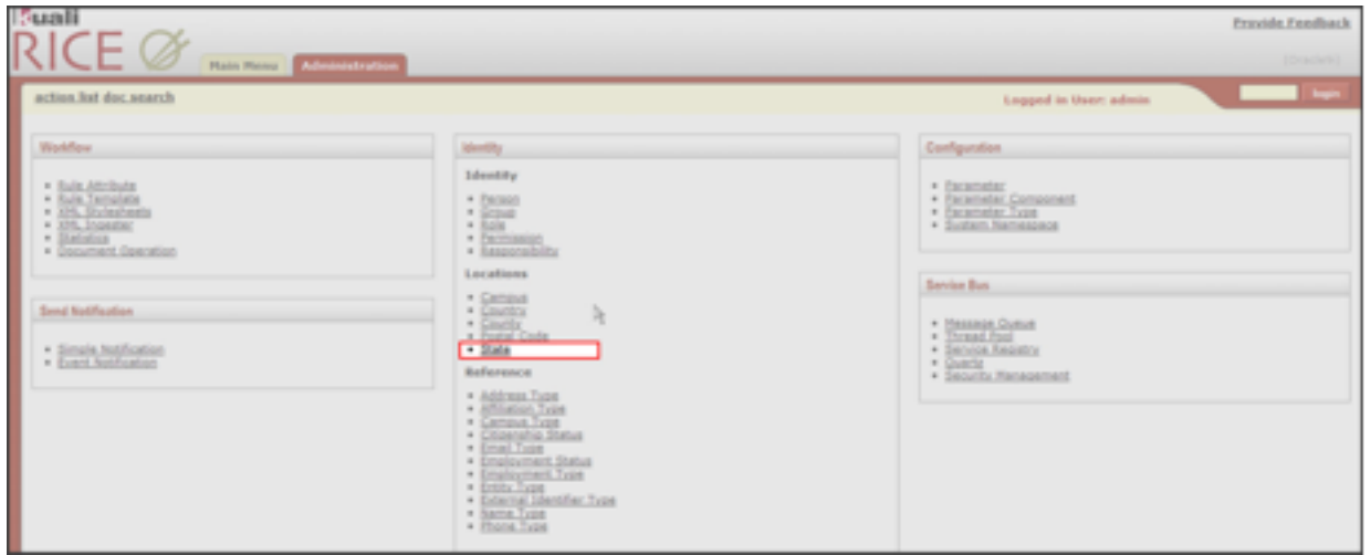
Figure 11.31. State Lookup
