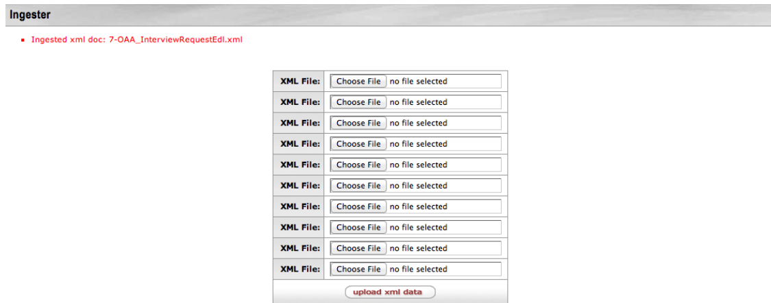
Figure 3.6. Ingestion Complete
