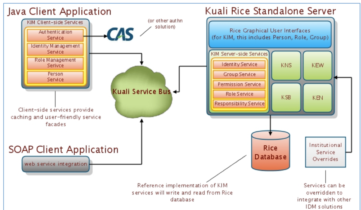
Figure 5.1. KIM Architecture
