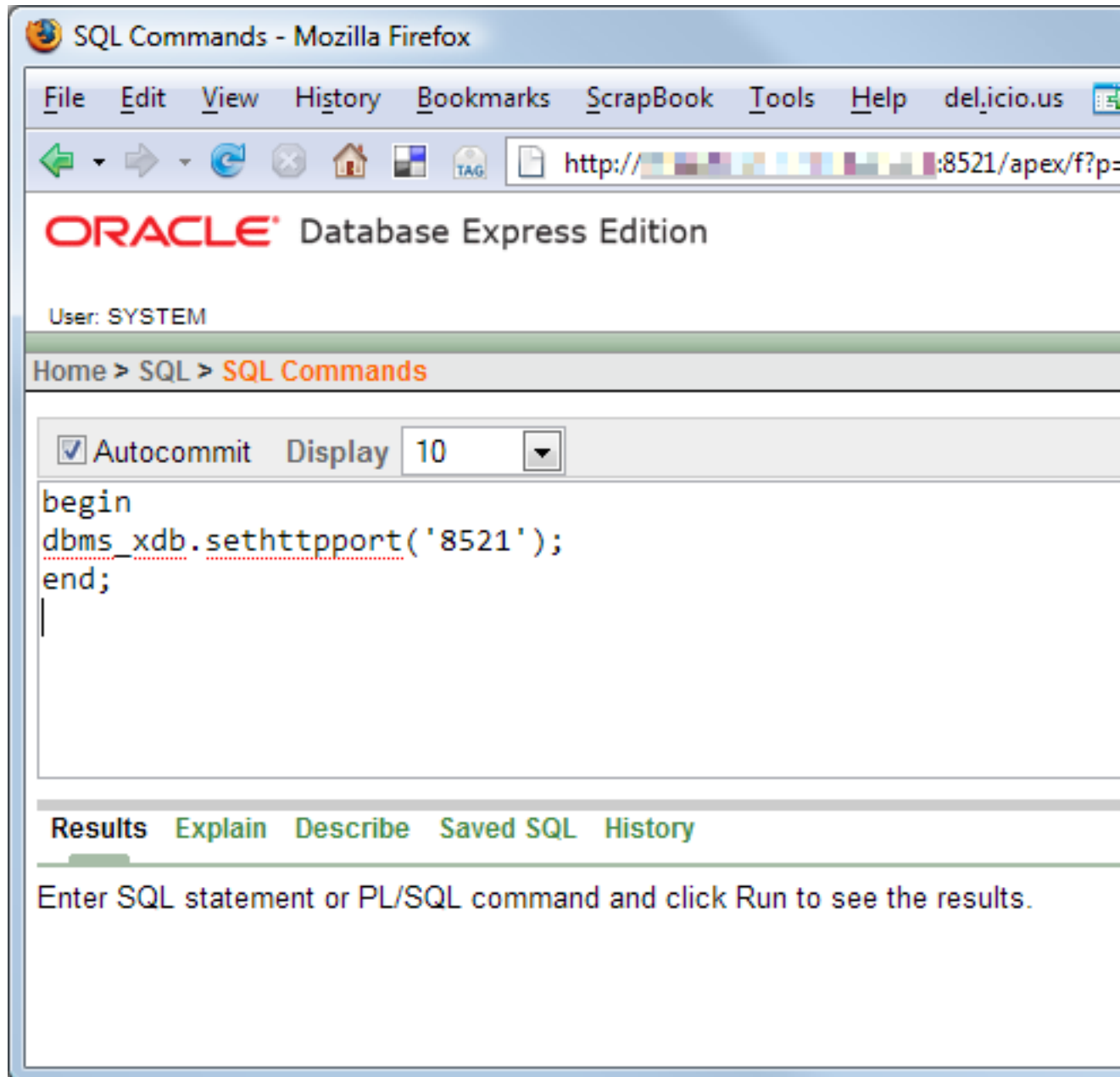
Figure 5.1. Oracle XE admin webapp
