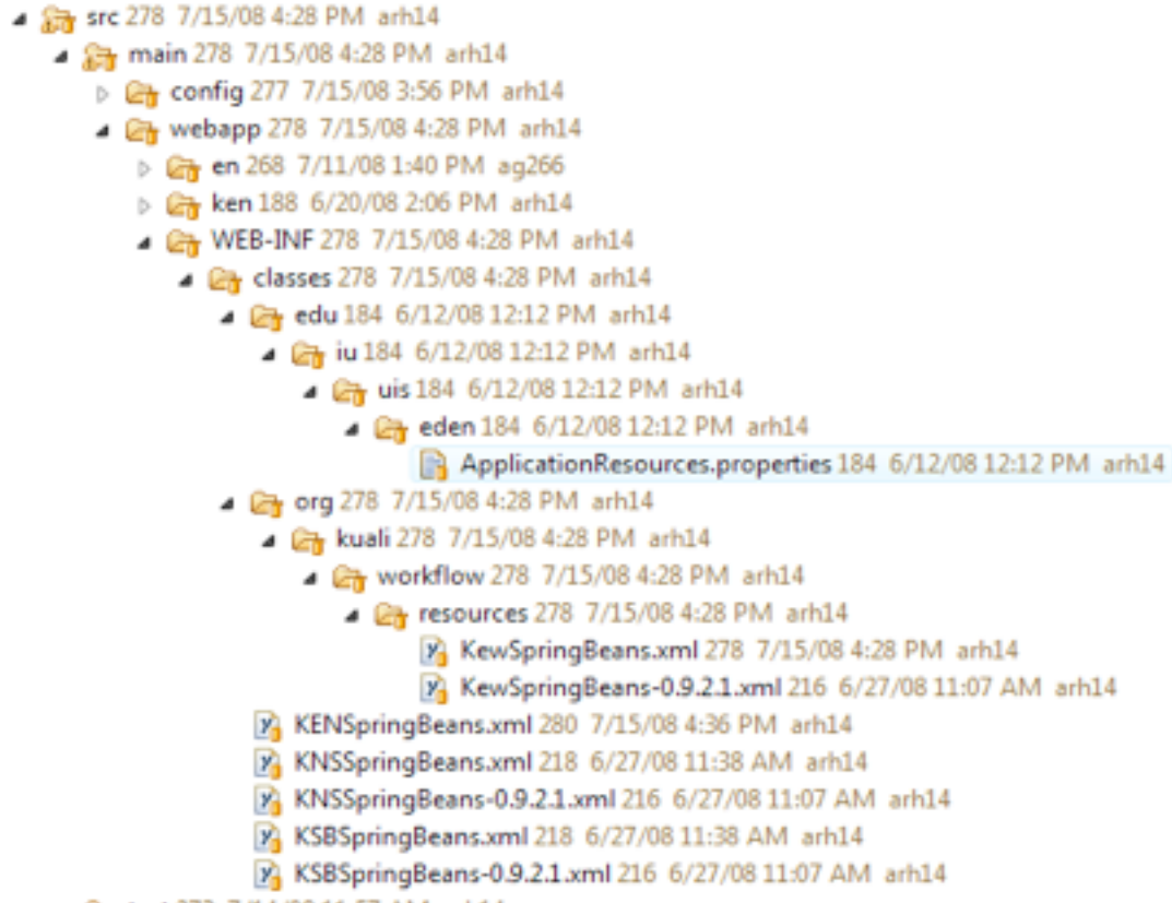
Figure 6.3. Application Resources Properties Tree
