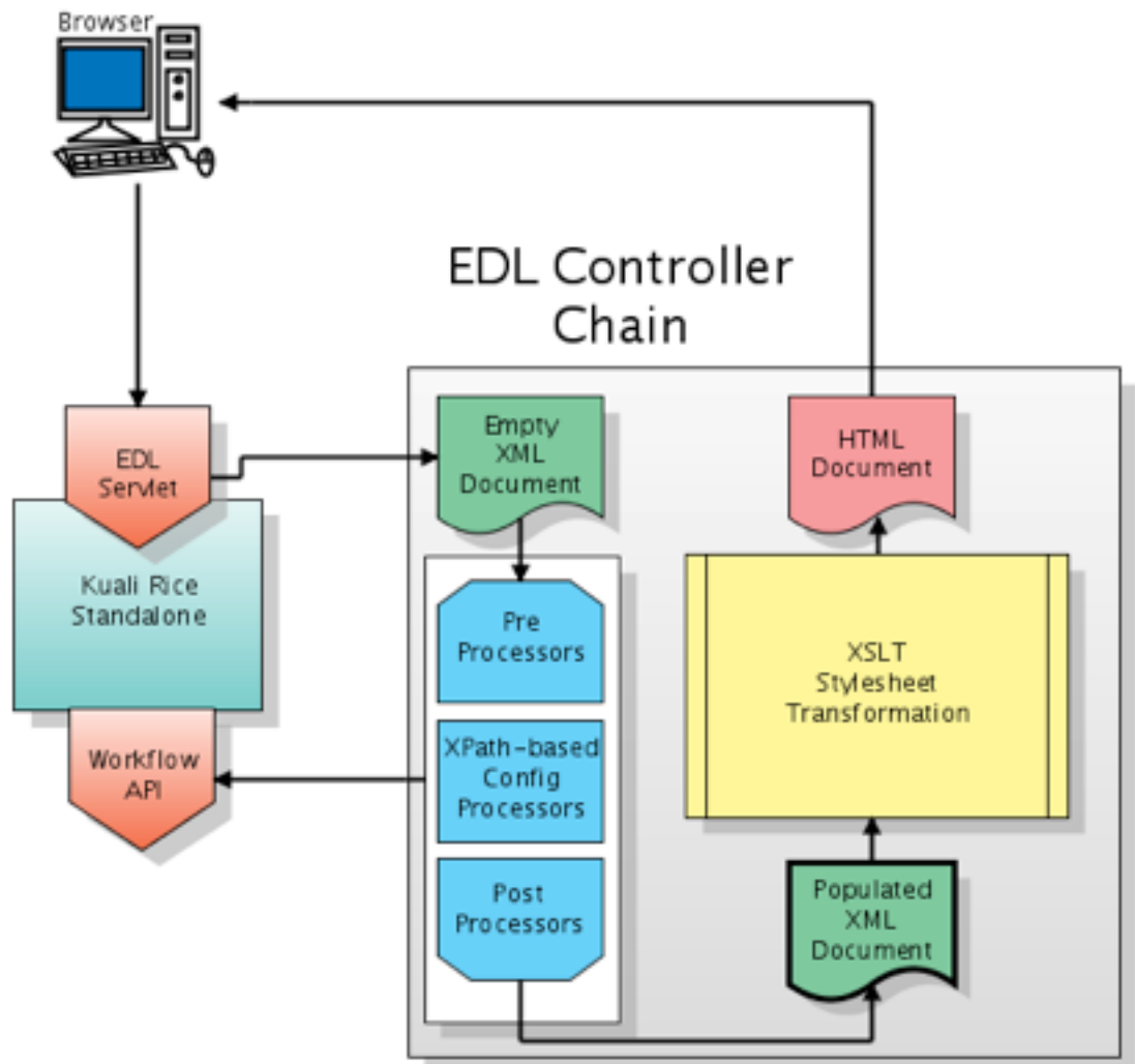
Figure 3.11. EDL Controller Chain
