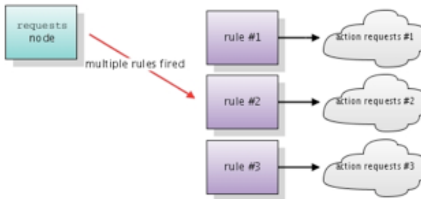
Figure 3.10. Activation Type
