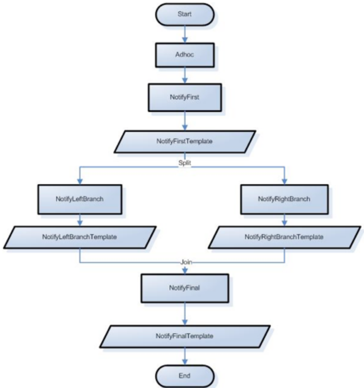
Figure 3.9. NotificationTest Workflow
