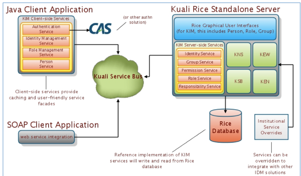
Figure 4.1. KIM Architecture
