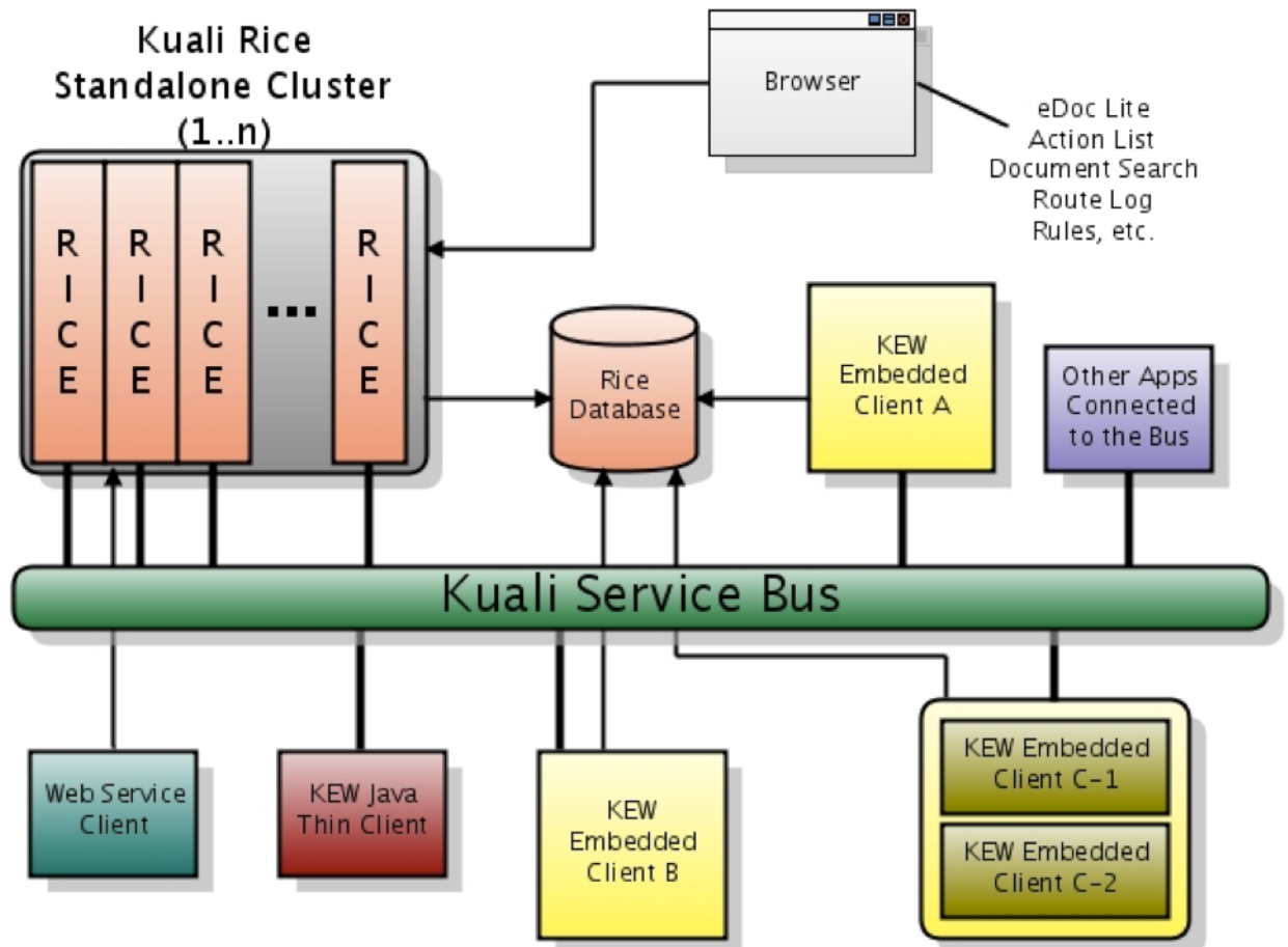
Figure 3.1. Kuali Rice 2.0.0-b2-SNAPSHOT Architectural Diagram
