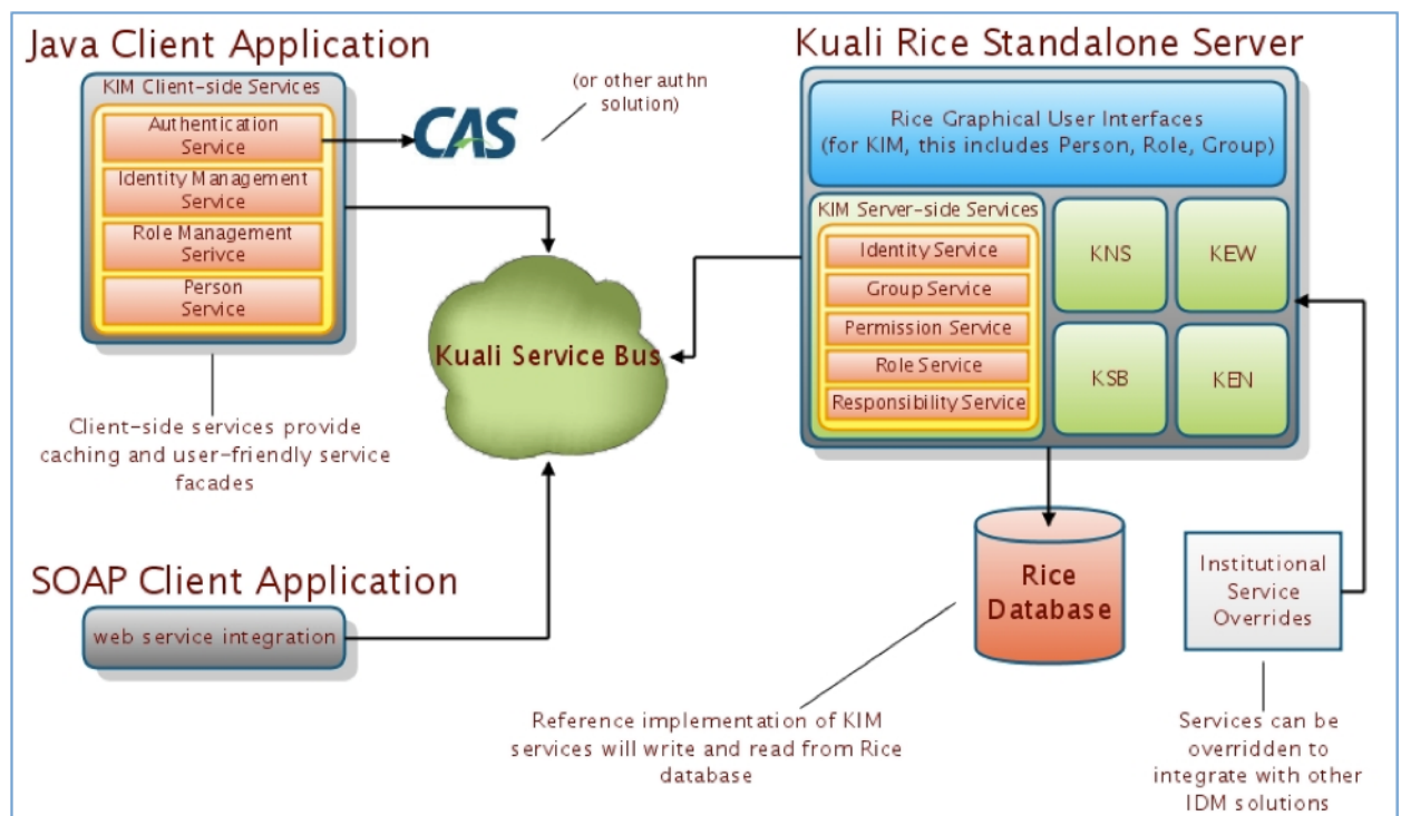
Figure 4.1. KIM Architecture
