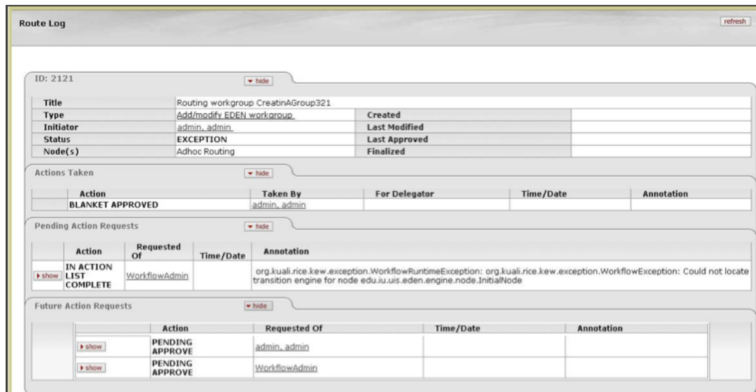
Figure 3.3. Route Log
