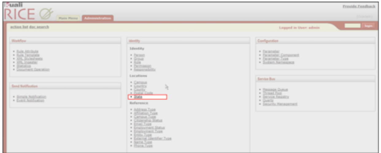
Figure 4.79. State Lookup
