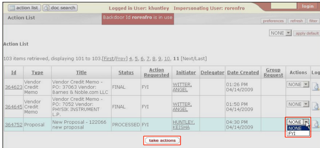
Figure 3.2. Action List
