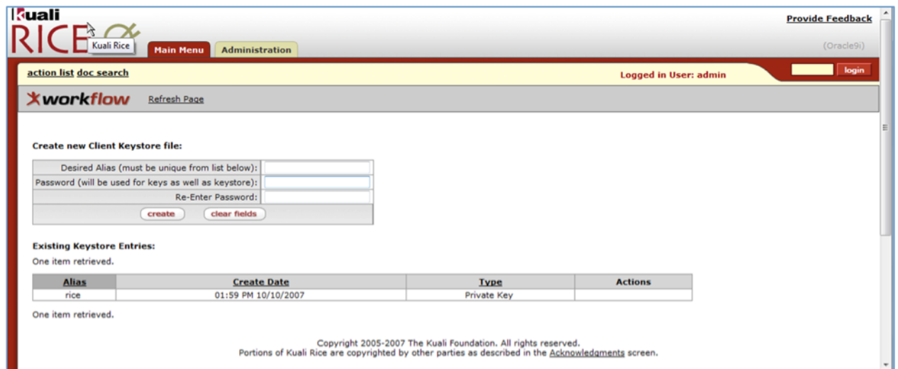
Figure 8.12. Create Keystore
