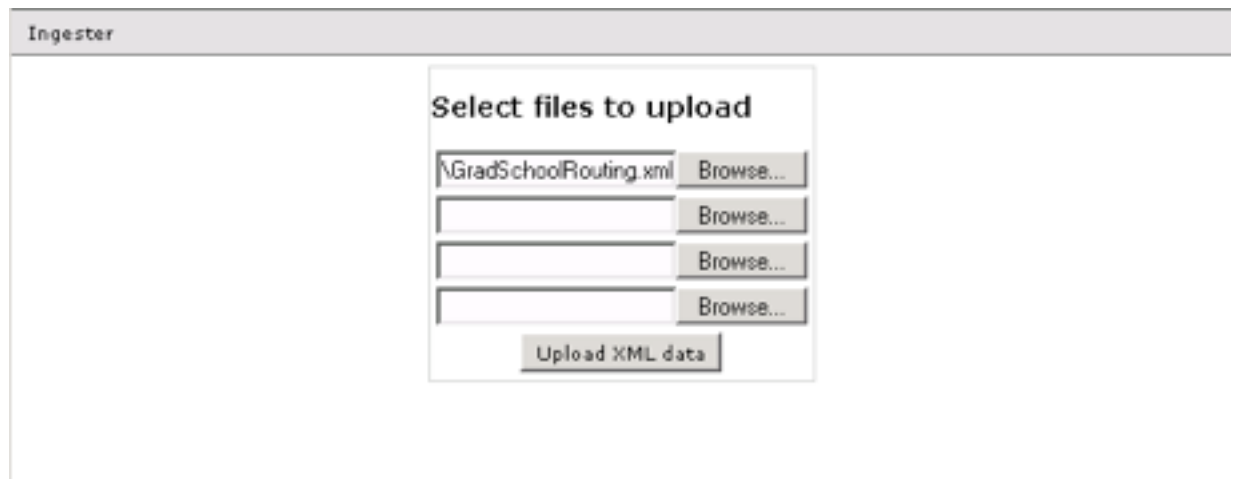
Figure 3.5. Ingestor
